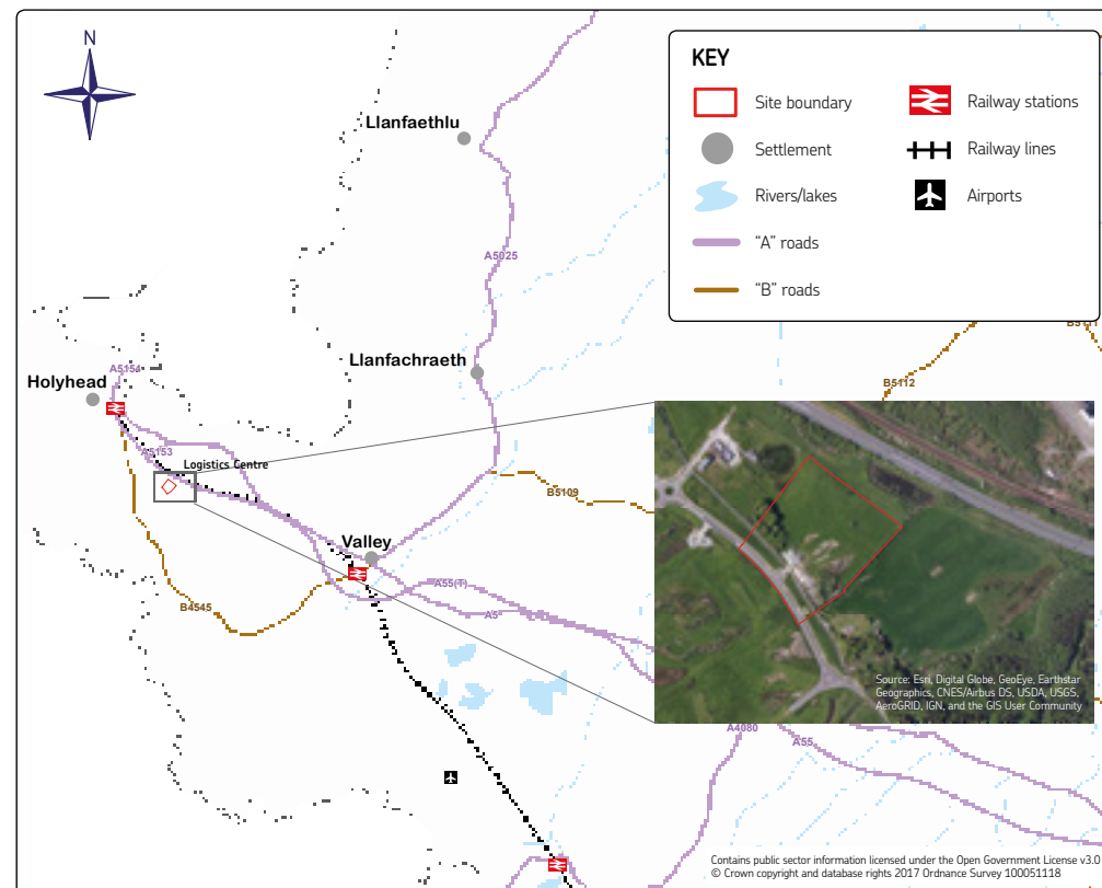
Logistics Centre preferred location – Parc Cybi
