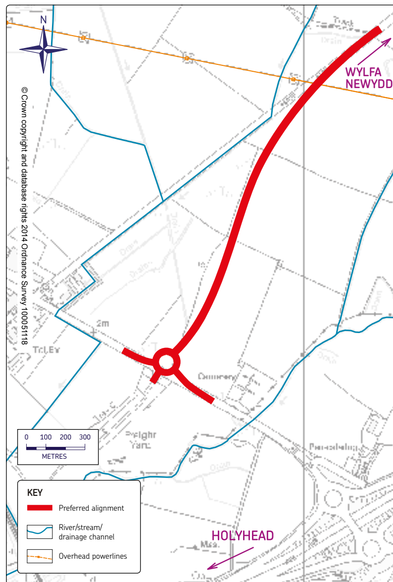
Indicative proposed highway alignment – Valley
