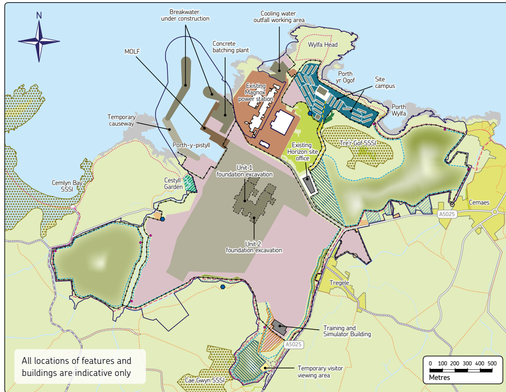
Completion of earthworks for Unit 1
